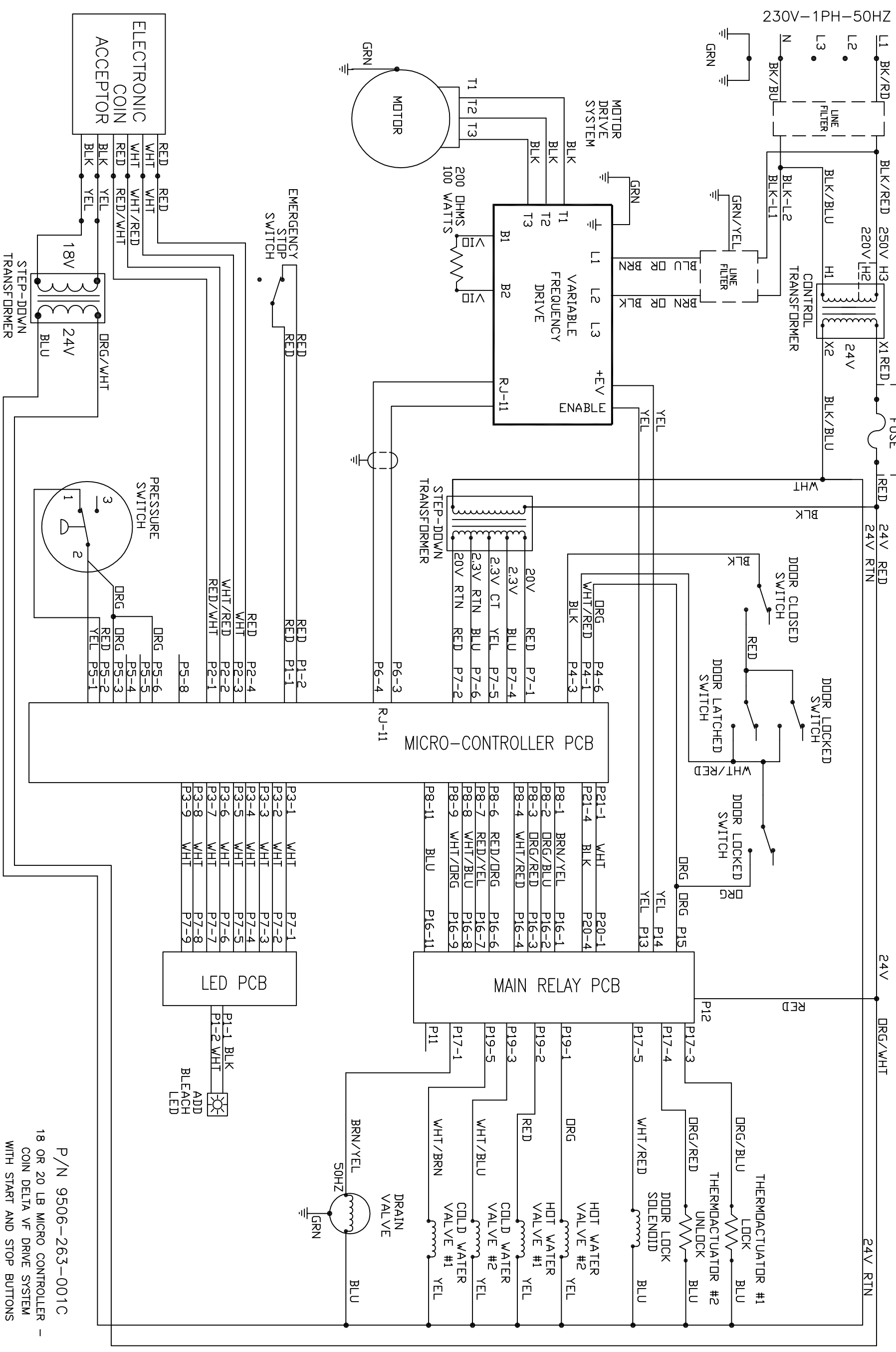
SCHEMATIC - 230V-1PH-50HZ
